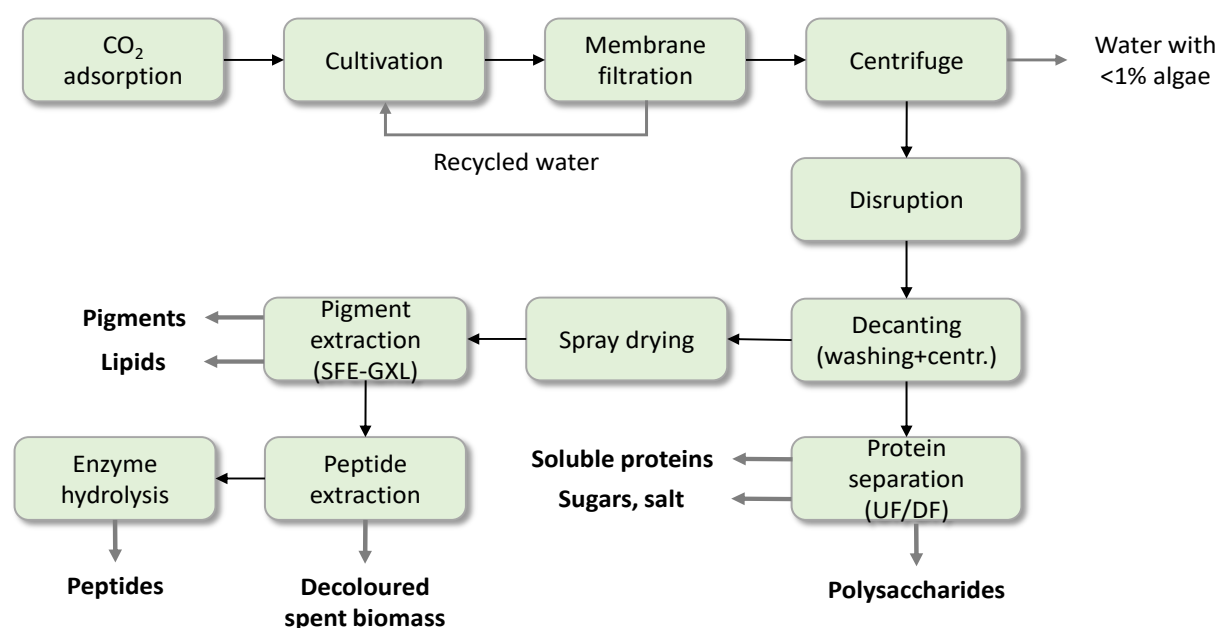
Figure 28. Multi product scenario MP1 protein-pigment-peptides
