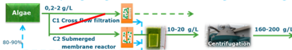
Figure 8. Schematic overview of different approaches for harvesting and medium recycling.
